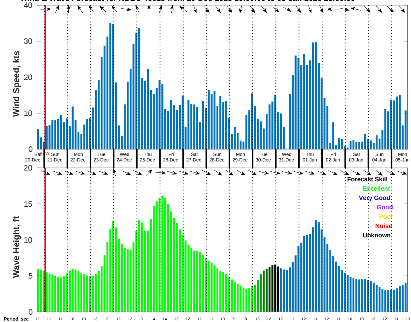
Wind & Wave Forecast for NDBC 46028 from 20-Dec-2025 16:00:00 to 05-Jan-2026 16:00:00
