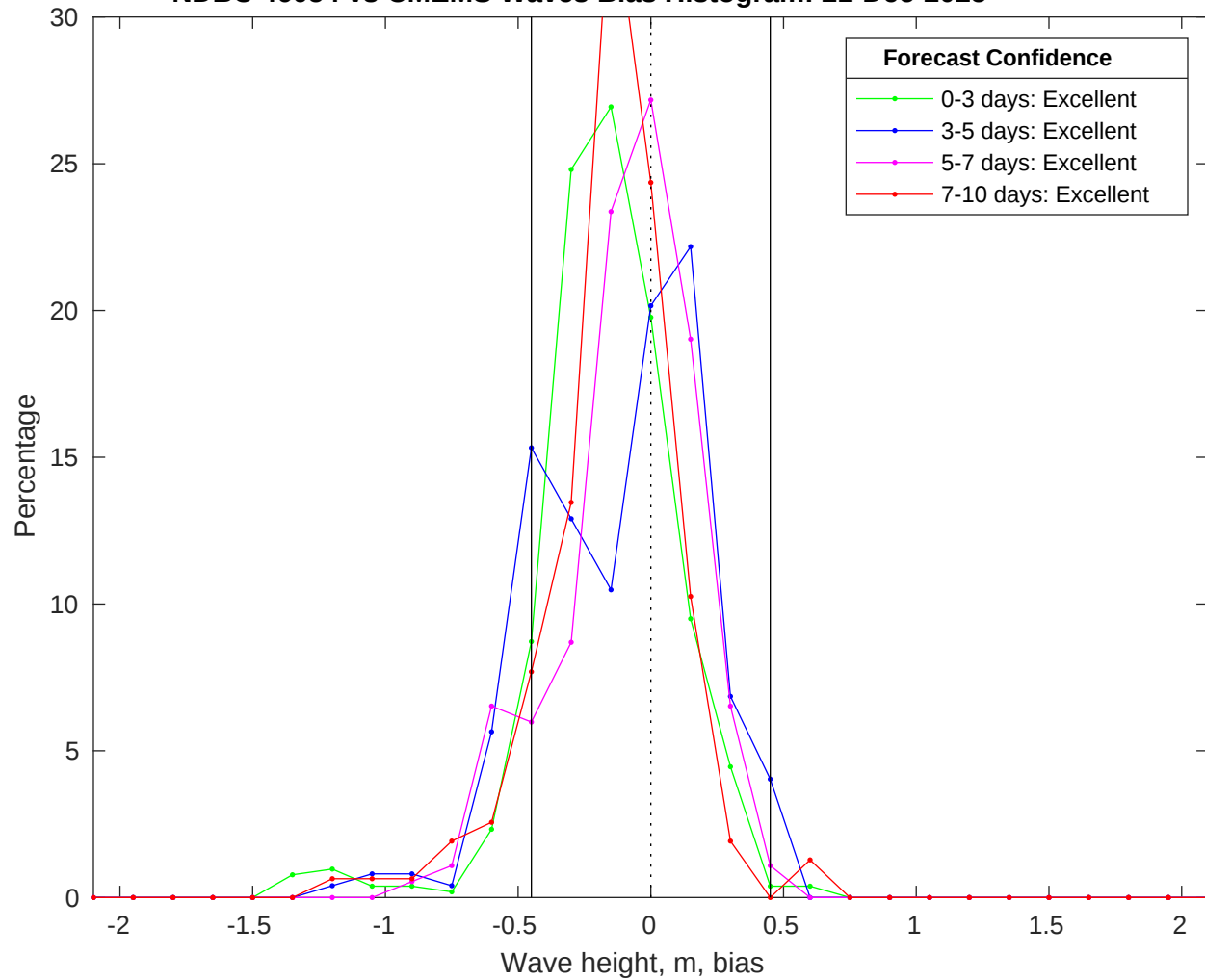
NDBC 46054 vs CMEMS Waves Bias Histogram: 21-Dec-2025
