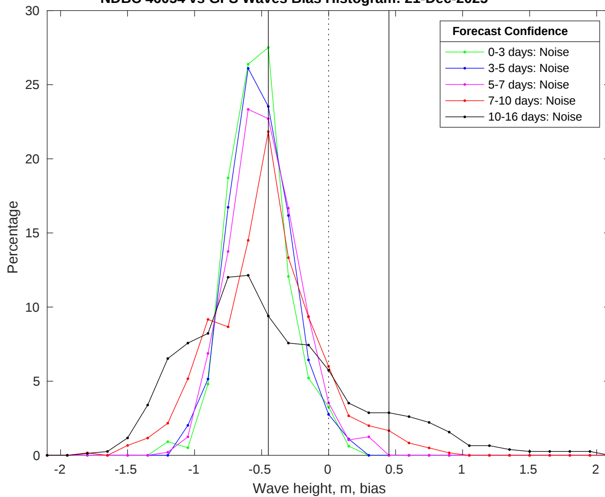
NDBC 46054 vs GFS Waves Bias Histogram: 21-Dec-2025
