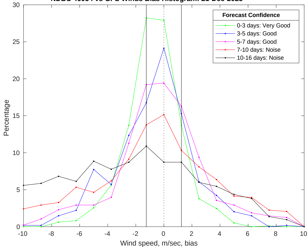
NDBC 46054 vs GFS Winds Bias Histogram: 21-Dec-2025
