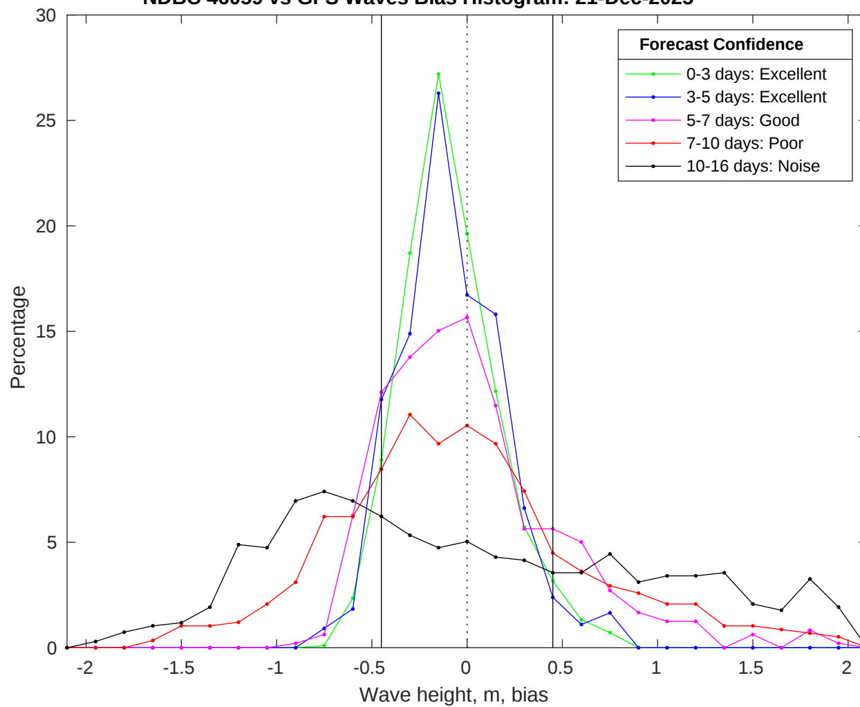
NDBC 46059 vs GFS Waves Bias Histogram: 21-Dec-2025
