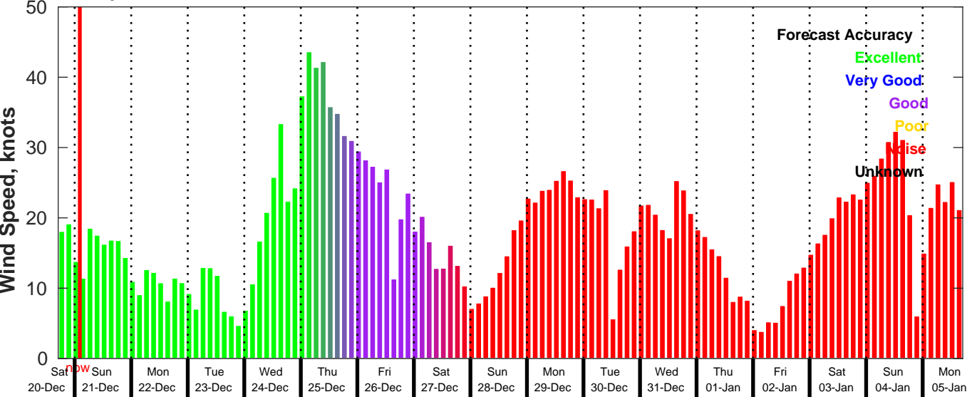
GFS Wind Speed Forecast for NDBC 46059 from 20-Dec-2025 17:00:00 to 05-Jan-2026 17:00:00
