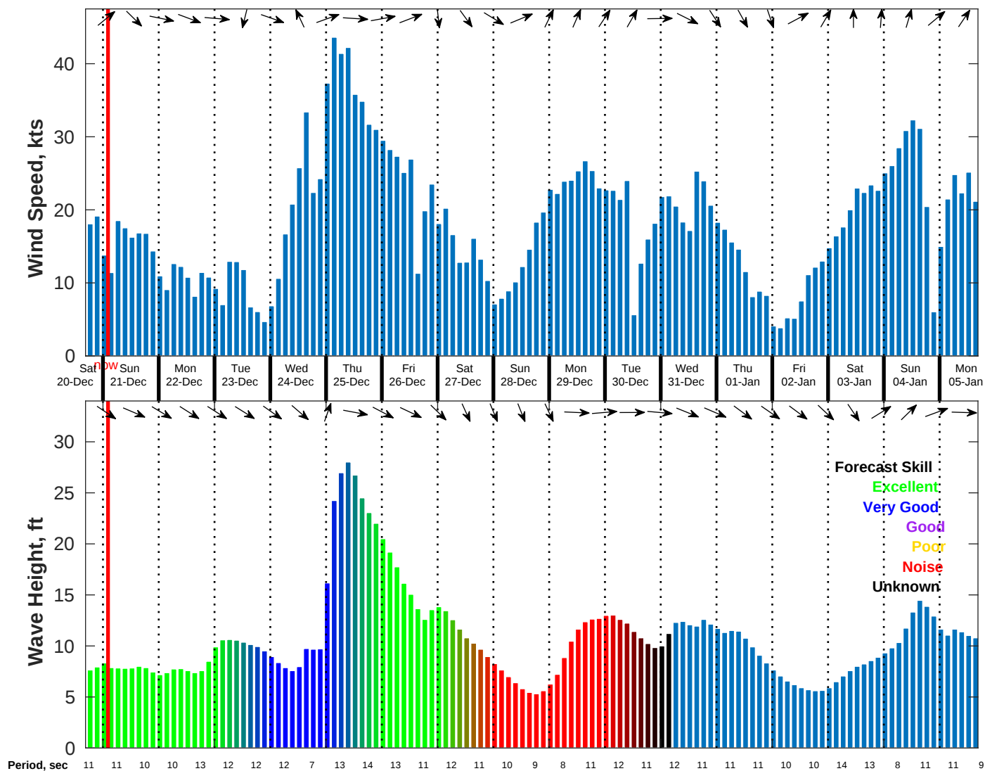
Wind & Wave Forecast for NDBC 46059 from 20-Dec-2025 17:00:00 to 05-Jan-2026 17:00:00
