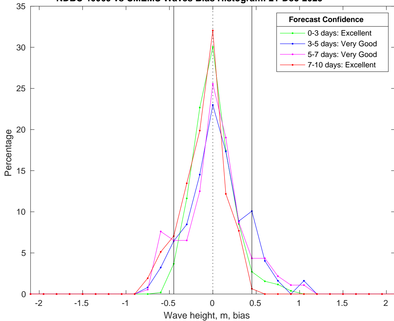
NDBC 46069 vs CMEMS Waves Bias Histogram: 21-Dec-2025
