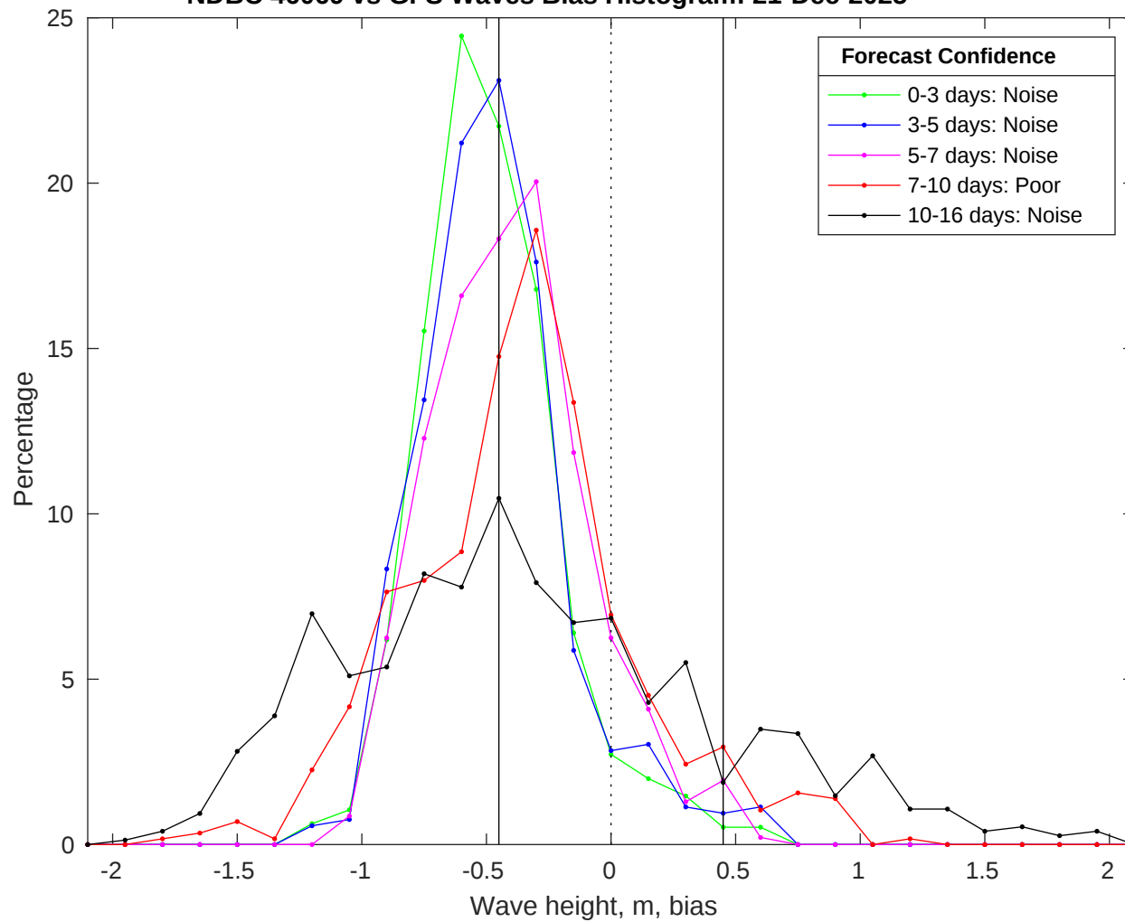
NDBC 46069 vs GFS Waves Bias Histogram: 21-Dec-2025
