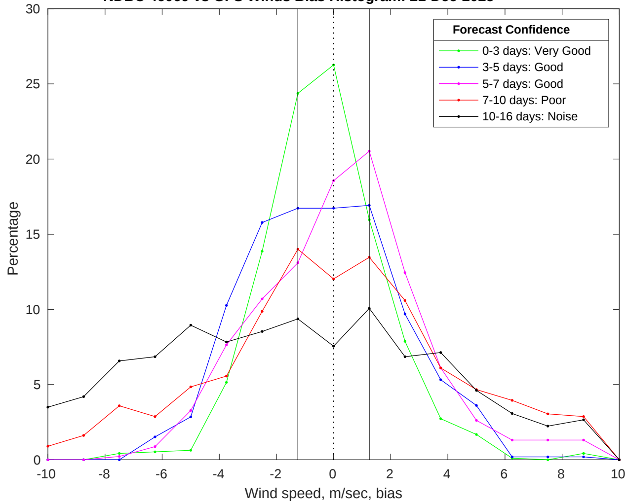
NDBC 46069 vs GFS Winds Bias Histogram: 21-Dec-2025
