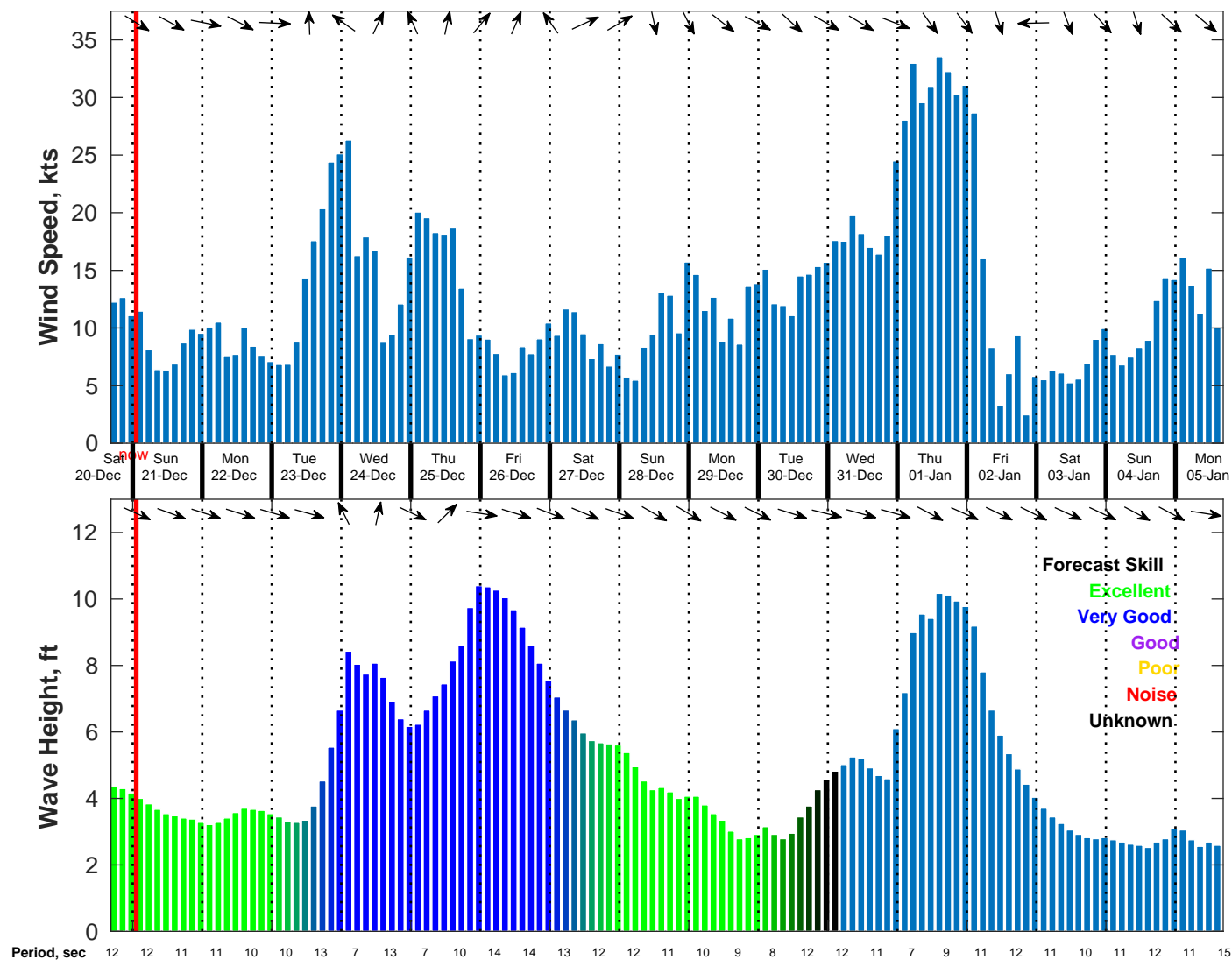
Wind & Wave Forecast for NDBC 46069 from 20-Dec-2025 16:00:00 to 05-Jan-2026 16:00:00
