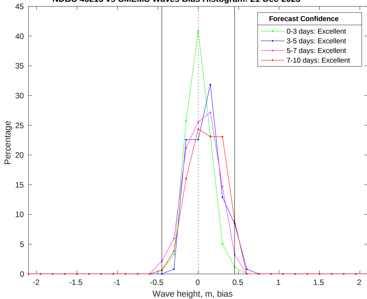
NDBC 46215 vs CMEMS Waves Bias Histogram: 21-Dec-2025
