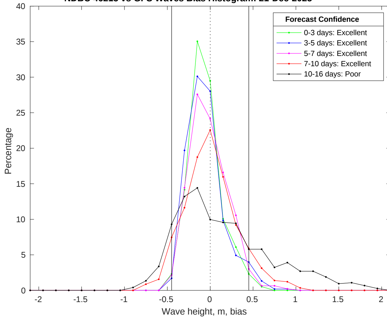
NDBC 46215 vs GFS Waves Bias Histogram: 21-Dec-2025
