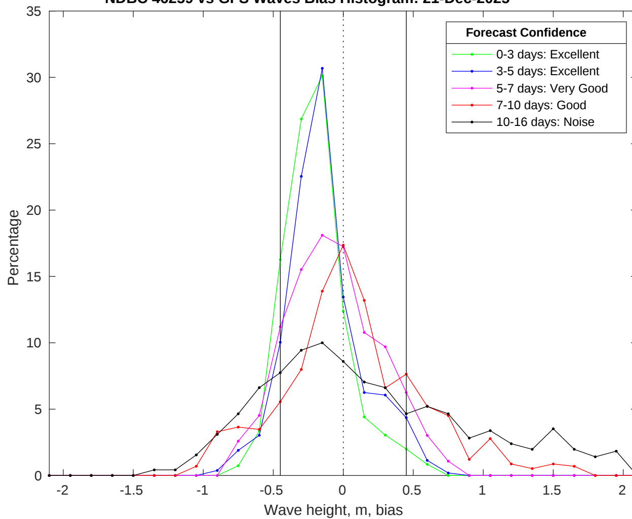
NDBC 46259 vs GFS Waves Bias Histogram: 21-Dec-2025
