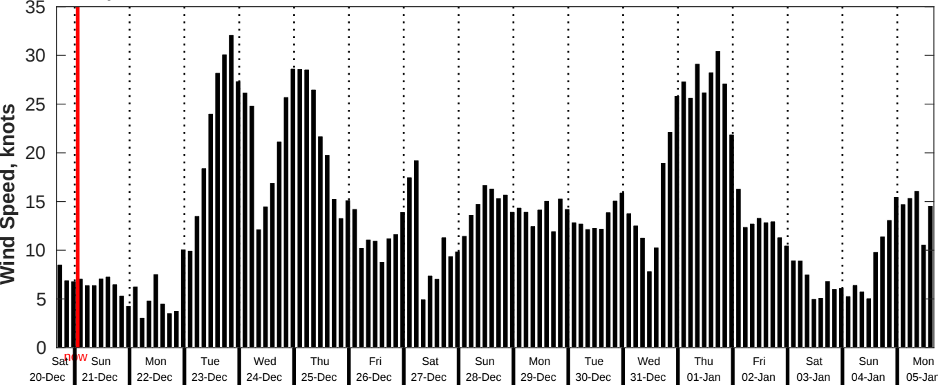
GFS Wind Speed Forecast for NDBC 46259 from 20-Dec-2025 16:00:00 to 05-Jan-2026 16:00:00
