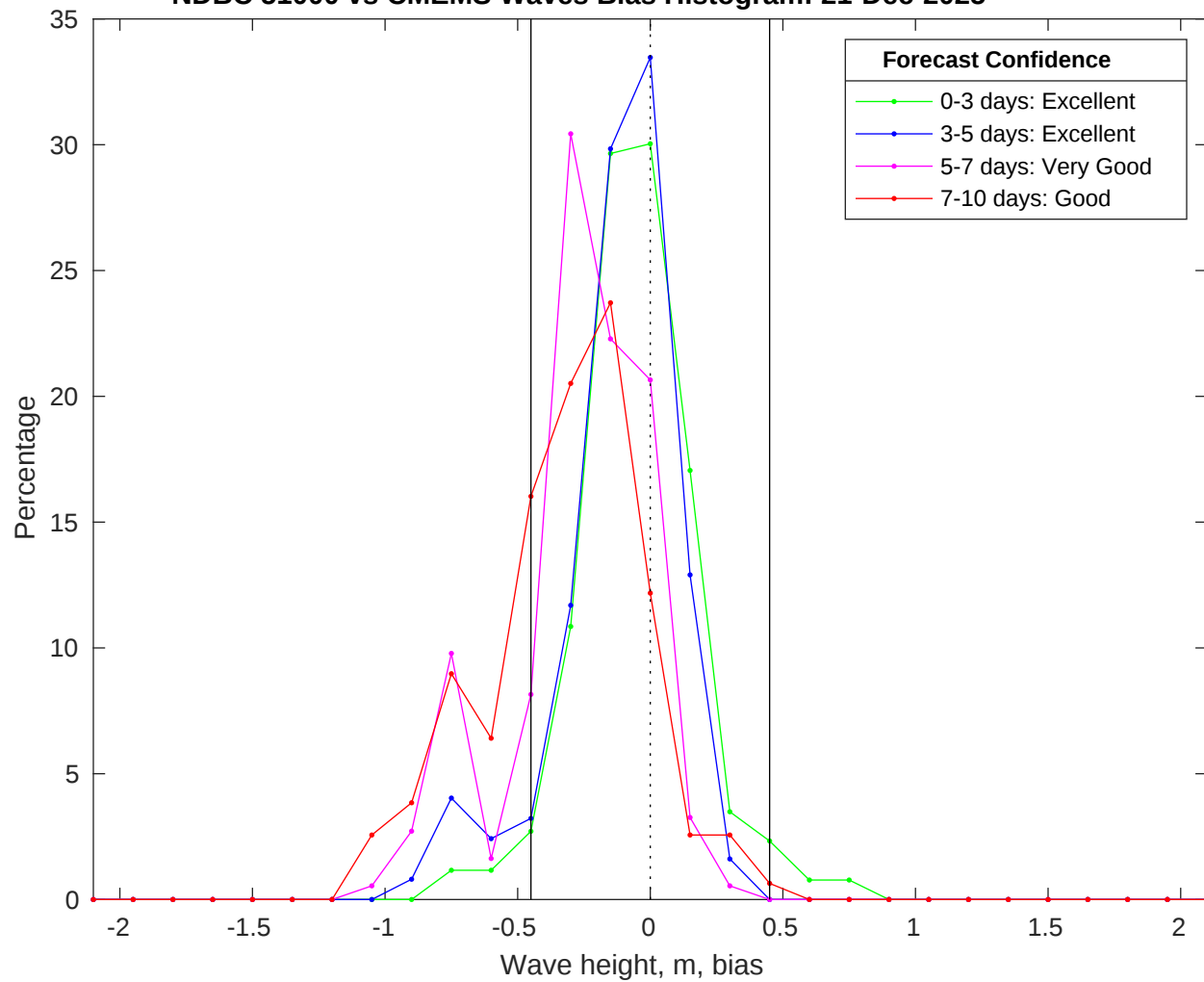
NDBC 51000 vs CMEMS Waves Bias Histogram: 21-Dec-2025
