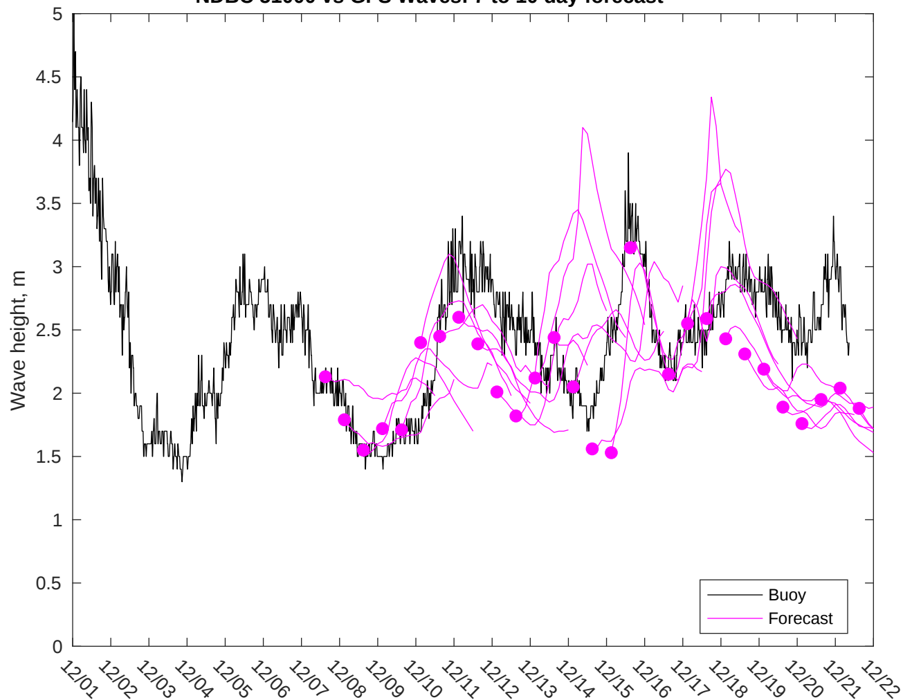
NDBC 51000 vs GFS Waves: 7 to 10 day forecast
