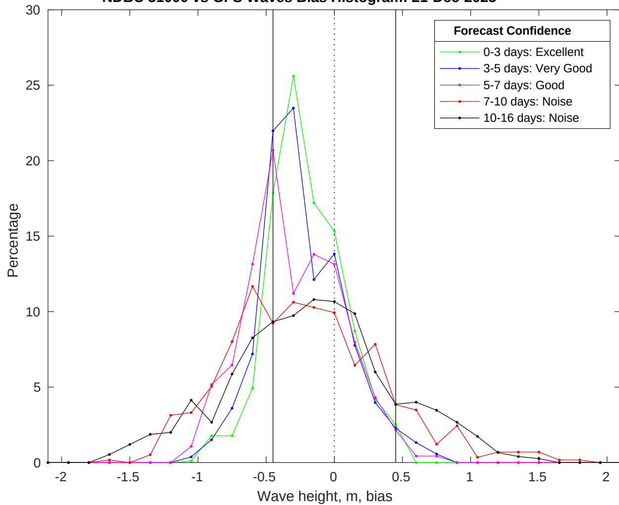
NDBC 51000 vs GFS Waves Bias Histogram: 21-Dec-2025
