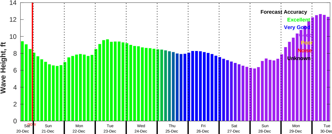
CMEMS Wave Forecast for NDBC 51000 from 20-Dec-2025 14:00:00 to 30-Dec-2025 14:00:00
