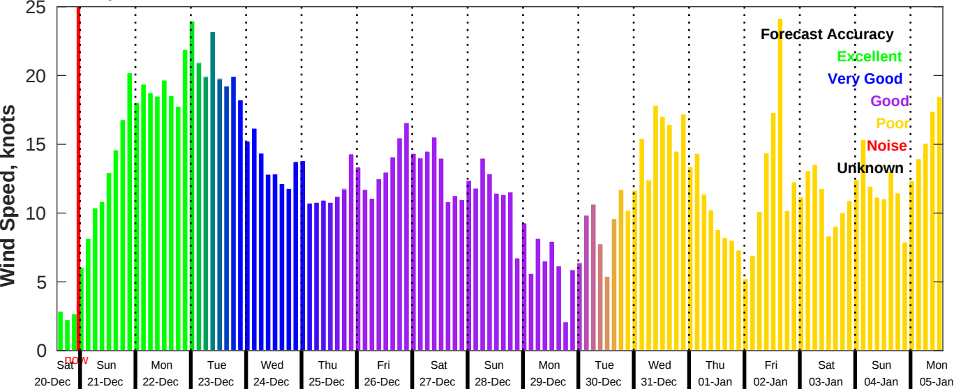
GFS Wind Speed Forecast for NDBC 51000 from 20-Dec-2025 14:00:00 to 05-Jan-2026 14:00:00
