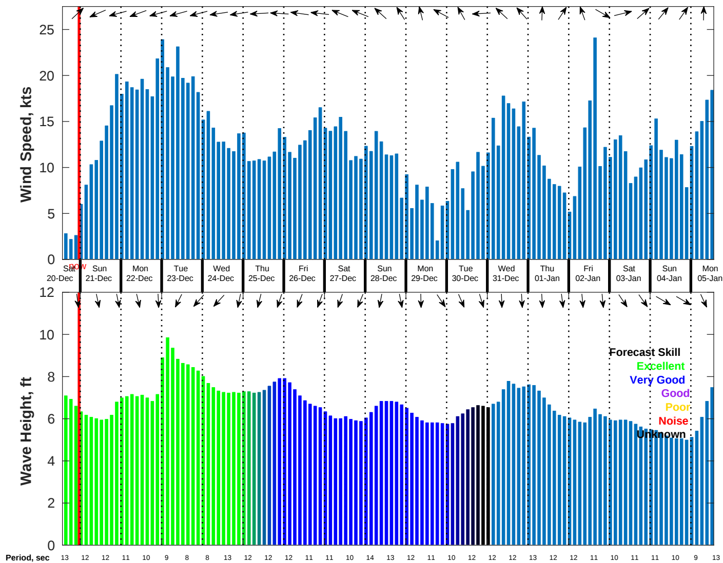
Wind & Wave Forecast for NDBC 51000 from 20-Dec-2025 14:00:00 to 05-Jan-2026 14:00:00
