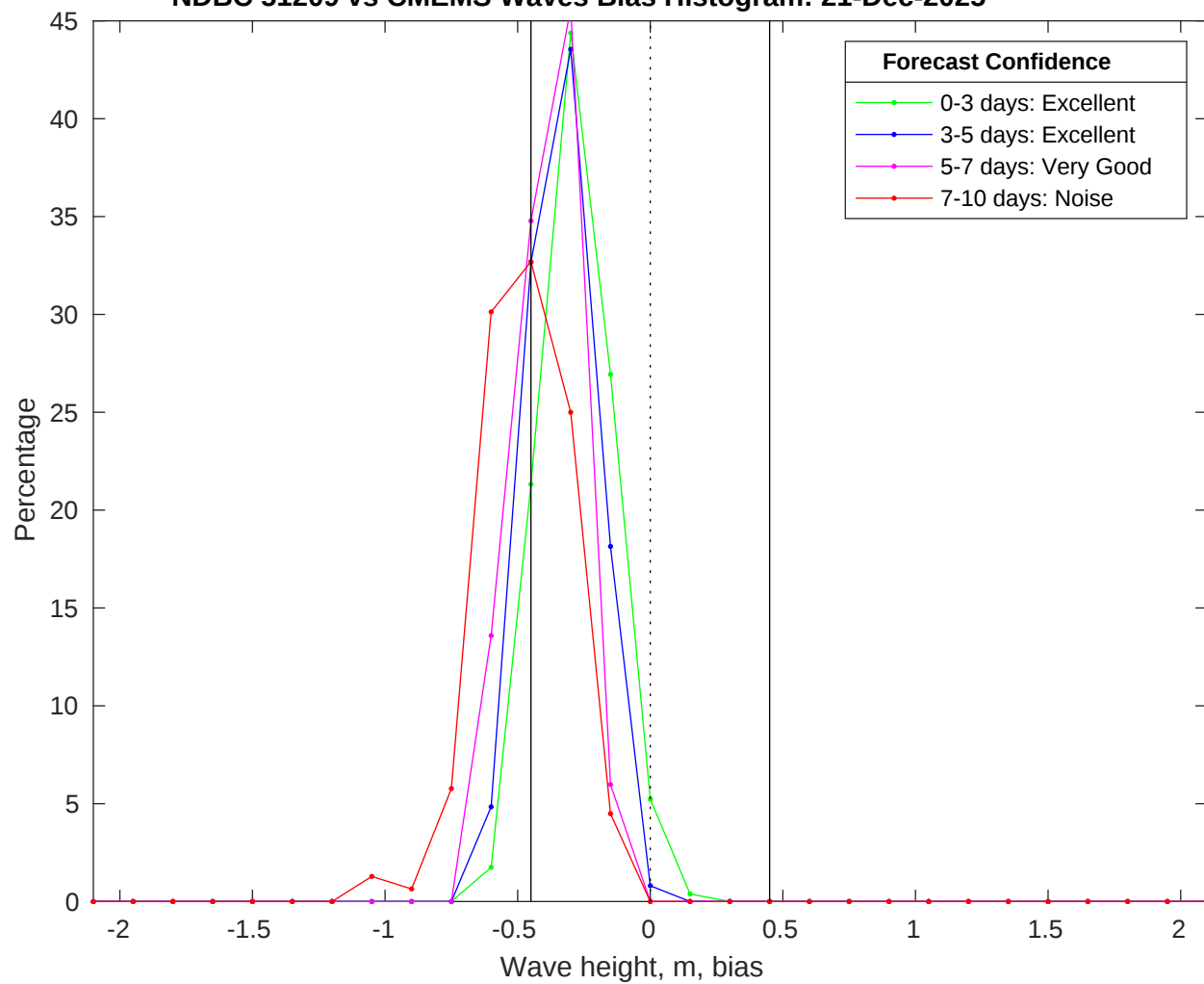
NDBC 51209 vs CMEMS Waves Bias Histogram: 21-Dec-2025
