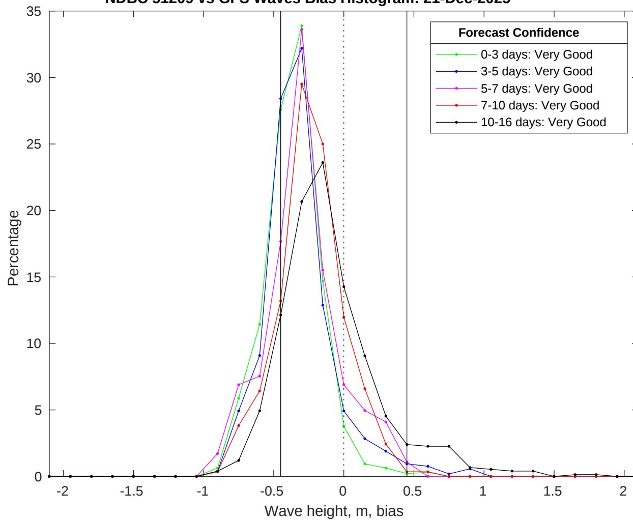
NDBC 51209 vs GFS Waves Bias Histogram: 21-Dec-2025
