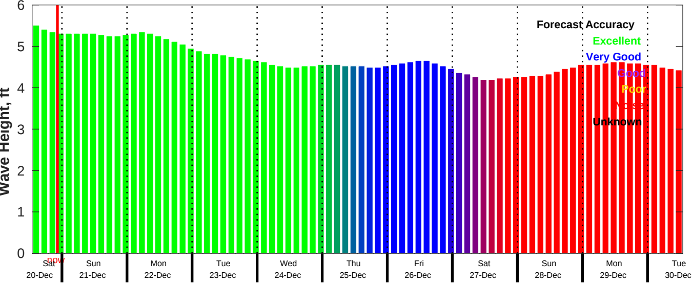
CMEMS Wave Forecast for NDBC 51209 from 20-Dec-2025 13:00:00 to 30-Dec-2025 13:00:00
