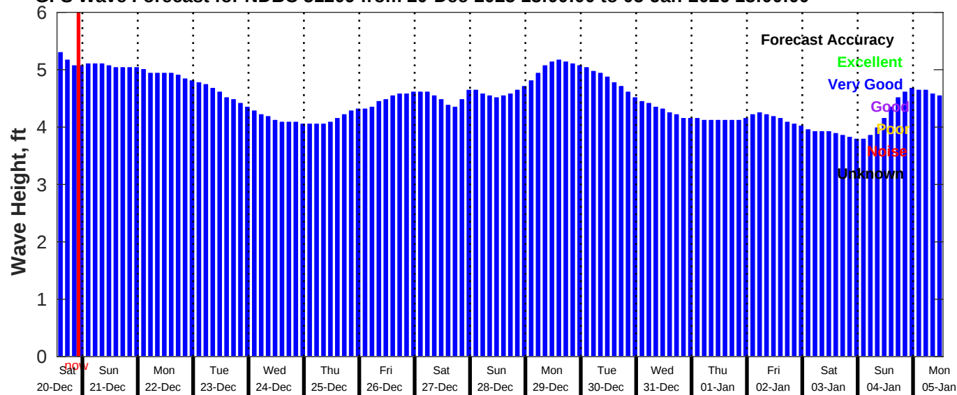
GFS Wave Forecast for NDBC 51209 from 20-Dec-2025 13:00:00 to 05-Jan-2026 13:00:00
