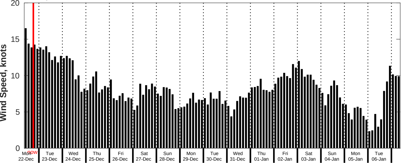
GFS Wind Speed Forecast for NDBC 52212 from 21-Dec-2025 09:00:00 to 06-Jan-2026 09:00:00
