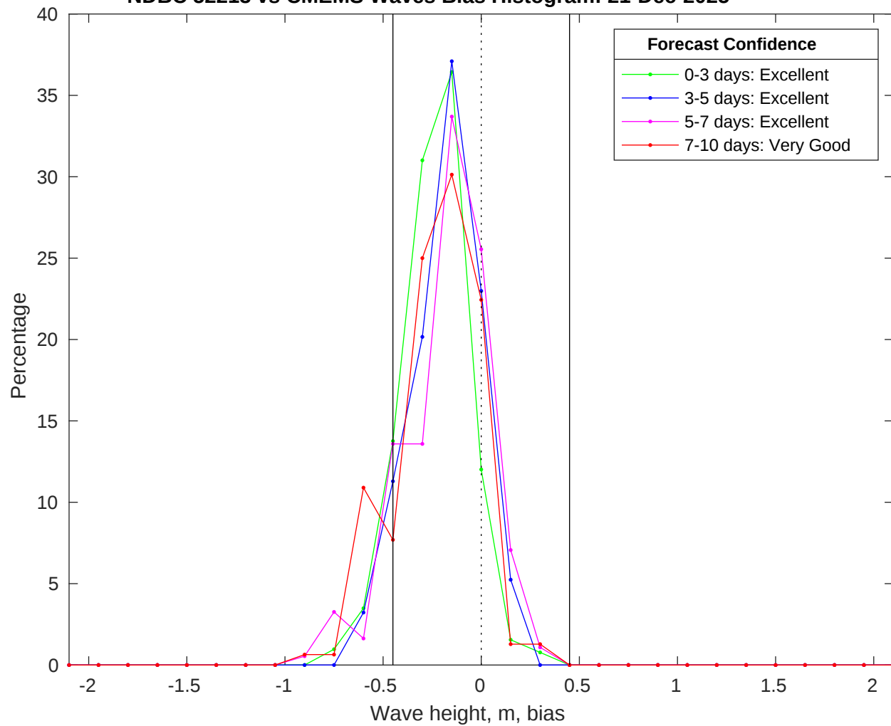
NDBC 52213 vs CMEMS Waves Bias Histogram: 21-Dec-2025
