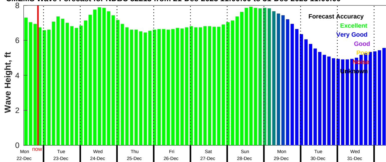
CMEMS Wave Forecast for NDBC 52213 from 21-Dec-2025 11:00:00 to 31-Dec-2025 11:00:00
