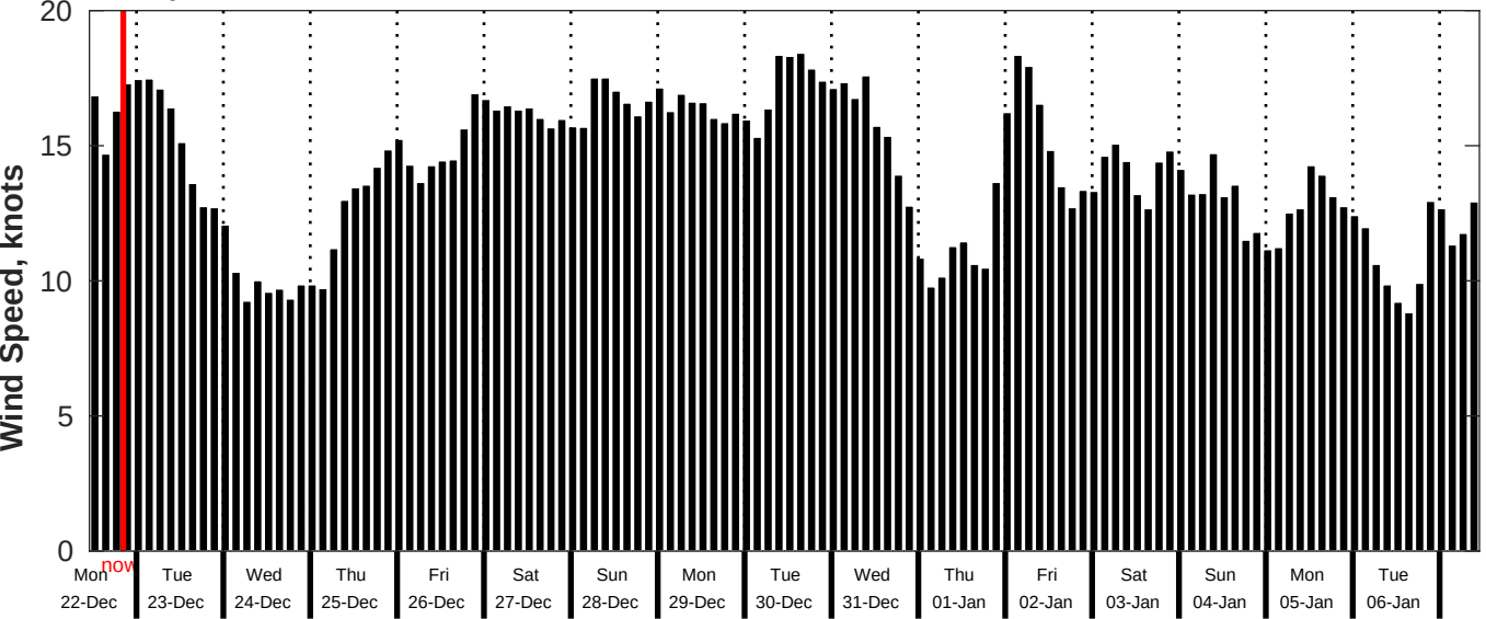
GFS Wind Speed Forecast for NDBC 52213 from 21-Dec-2025 11:00:00 to 06-Jan-2026 11:00:00
