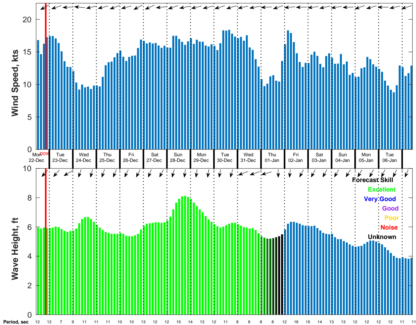
Wind & Wave Forecast for NDBC 52213 from 21-Dec-2025 11:00:00 to 06-Jan-2026 11:00:00
