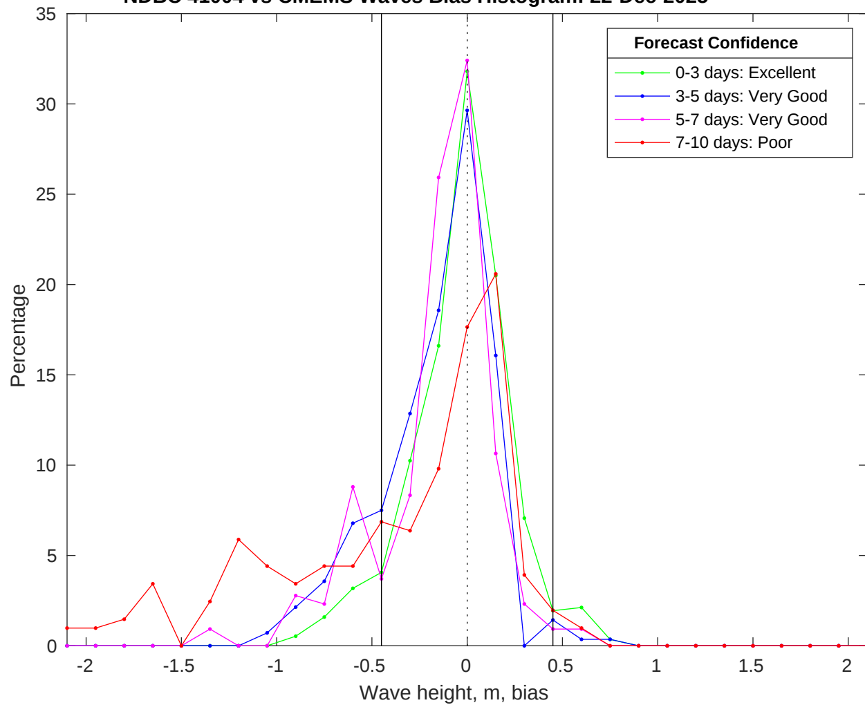
NDBC 41004 vs CMEMS Waves Bias Histogram: 22-Dec-2025
