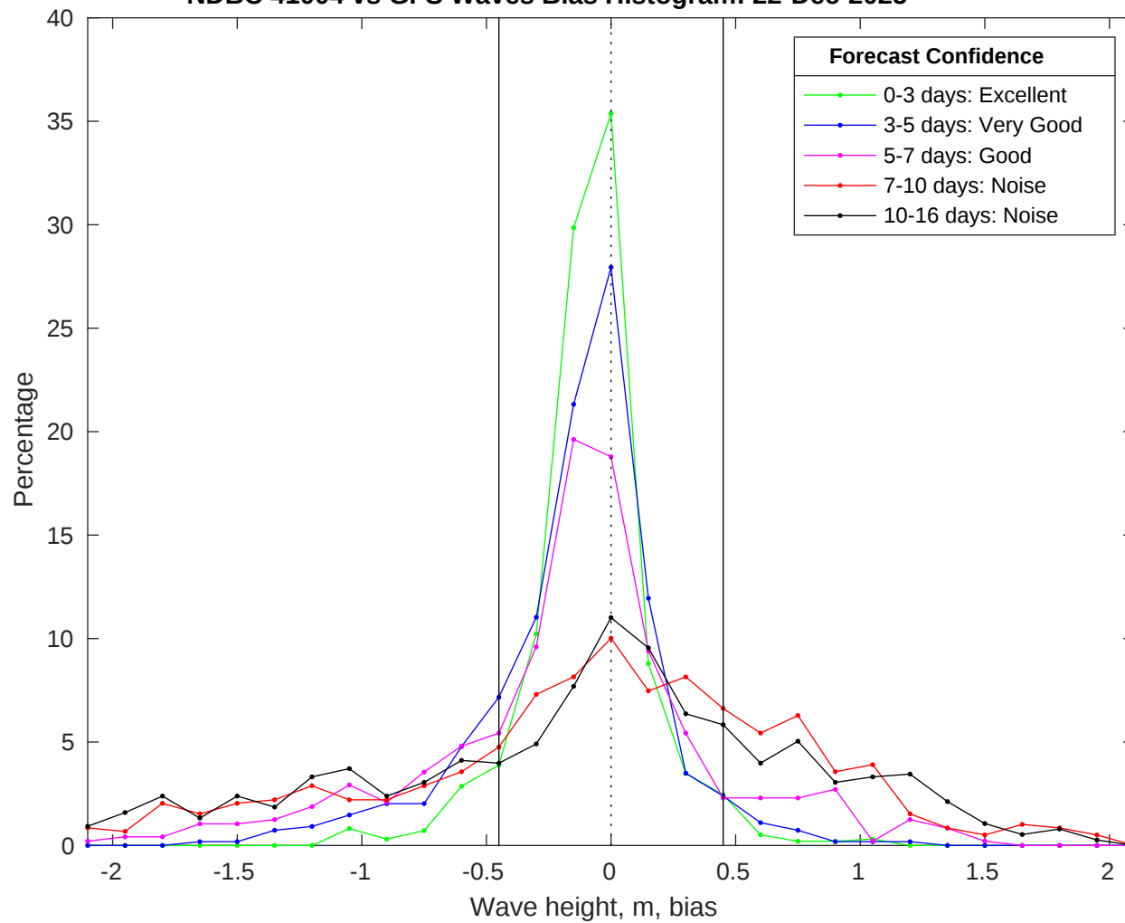
NDBC 41004 vs GFS Waves Bias Histogram: 22-Dec-2025
