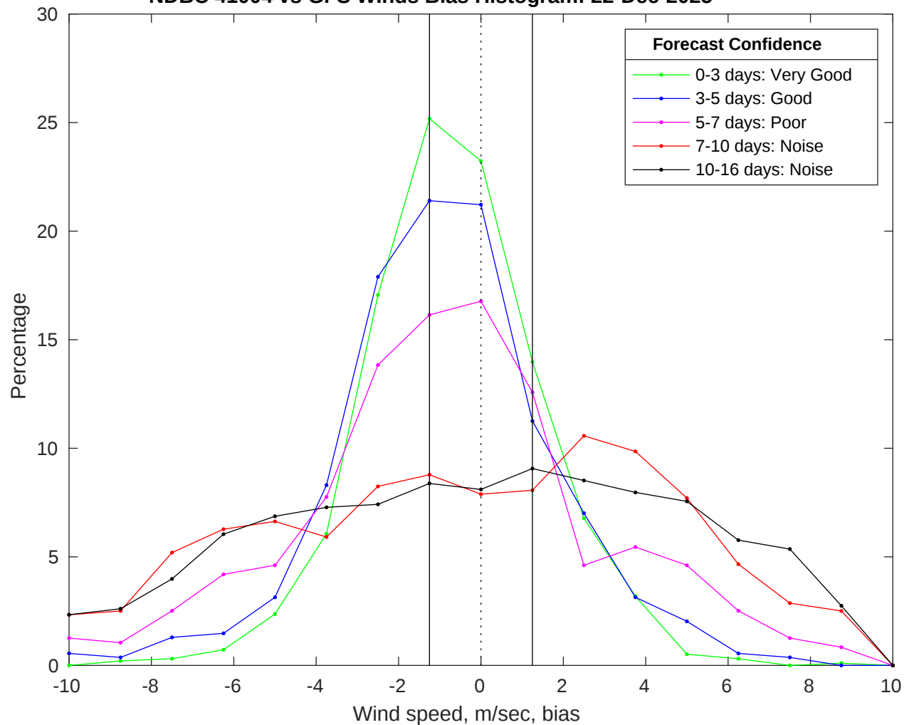
NDBC 41004 vs GFS Winds Bias Histogram: 22-Dec-2025
