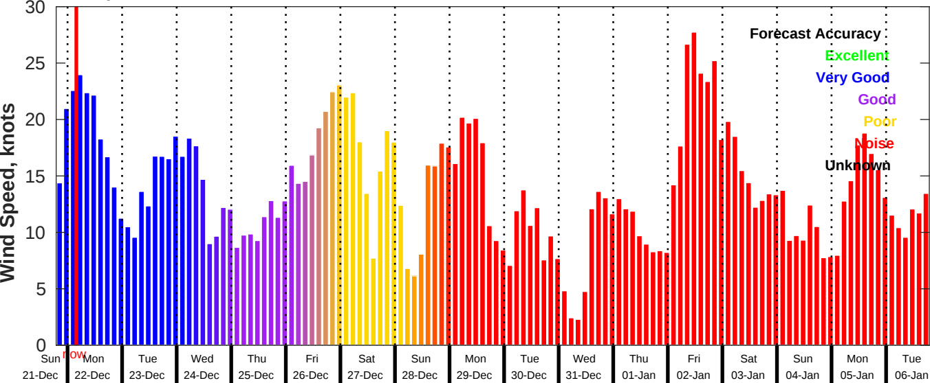
GFS Wind Speed Forecast for NDBC 41004 from 21-Dec-2025 19:00:00 to 06-Jan-2026 19:00:00
