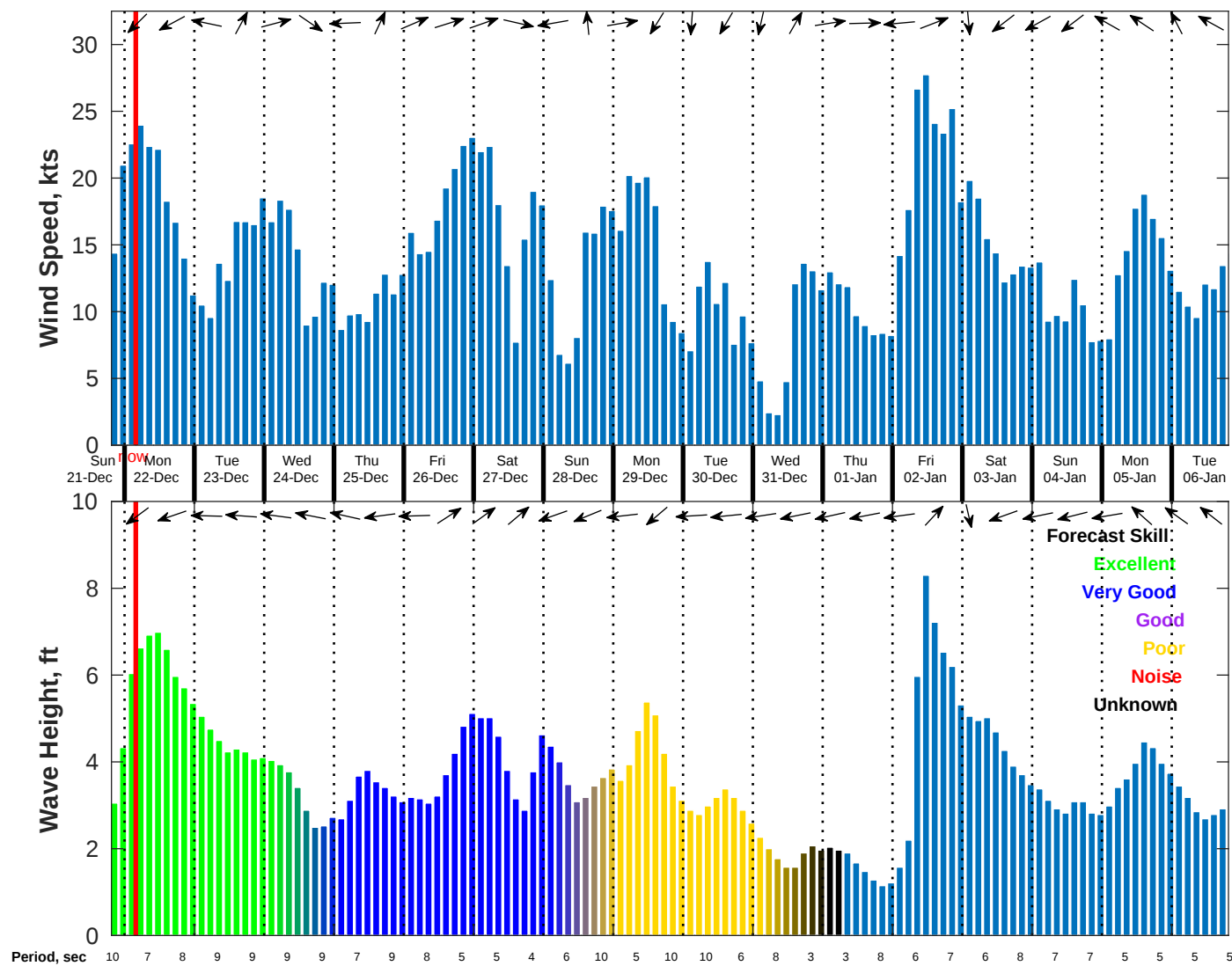
Wind & Wave Forecast for NDBC 41004 from 21-Dec-2025 19:00:00 to 06-Jan-2026 19:00:00
