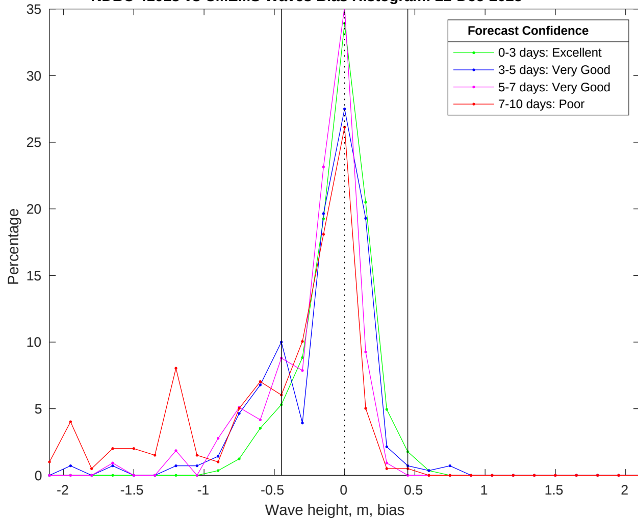
NDBC 41013 vs CMEMS Waves Bias Histogram: 22-Dec-2025
