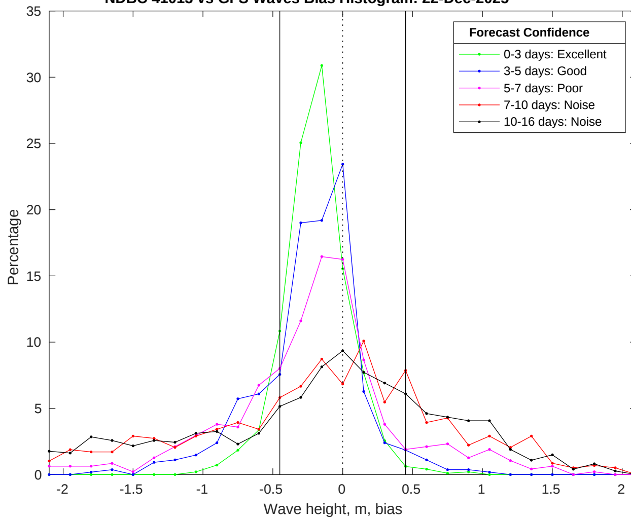
NDBC 41013 vs GFS Waves Bias Histogram: 22-Dec-2025
