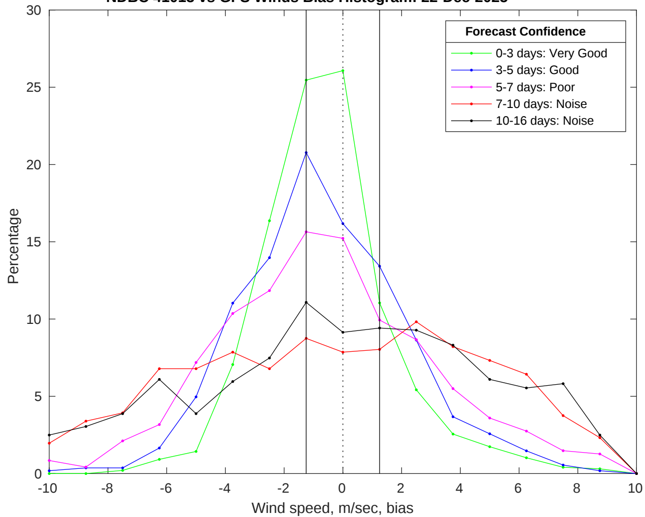
NDBC 41013 vs GFS Winds Bias Histogram: 22-Dec-2025
