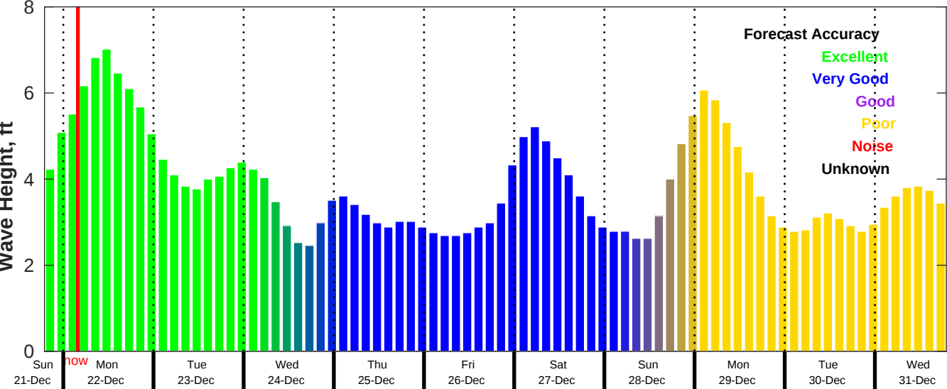
CMEMS Wave Forecast for NDBC 41013 from 21-Dec-2025 19:00:00 to 31-Dec-2025 19:00:00
