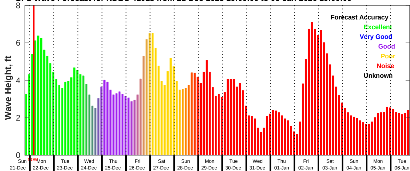
GFS Wave Forecast for NDBC 41013 from 21-Dec-2025 19:00:00 to 06-Jan-2026 19:00:00
