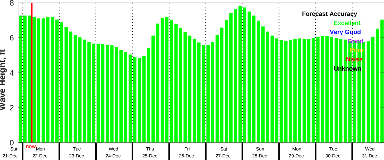
CMEMS Wave Forecast for NDBC 41040 from 21-Dec-2025 21:00:00 to 31-Dec-2025 21:00:00
