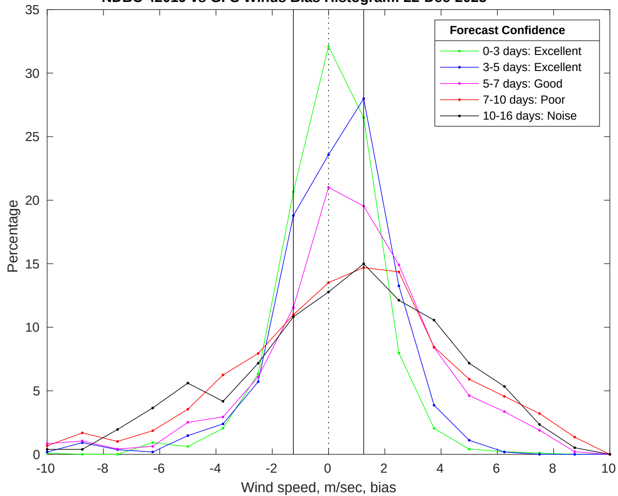
NDBC 42019 vs GFS Winds Bias Histogram: 22-Dec-2025
