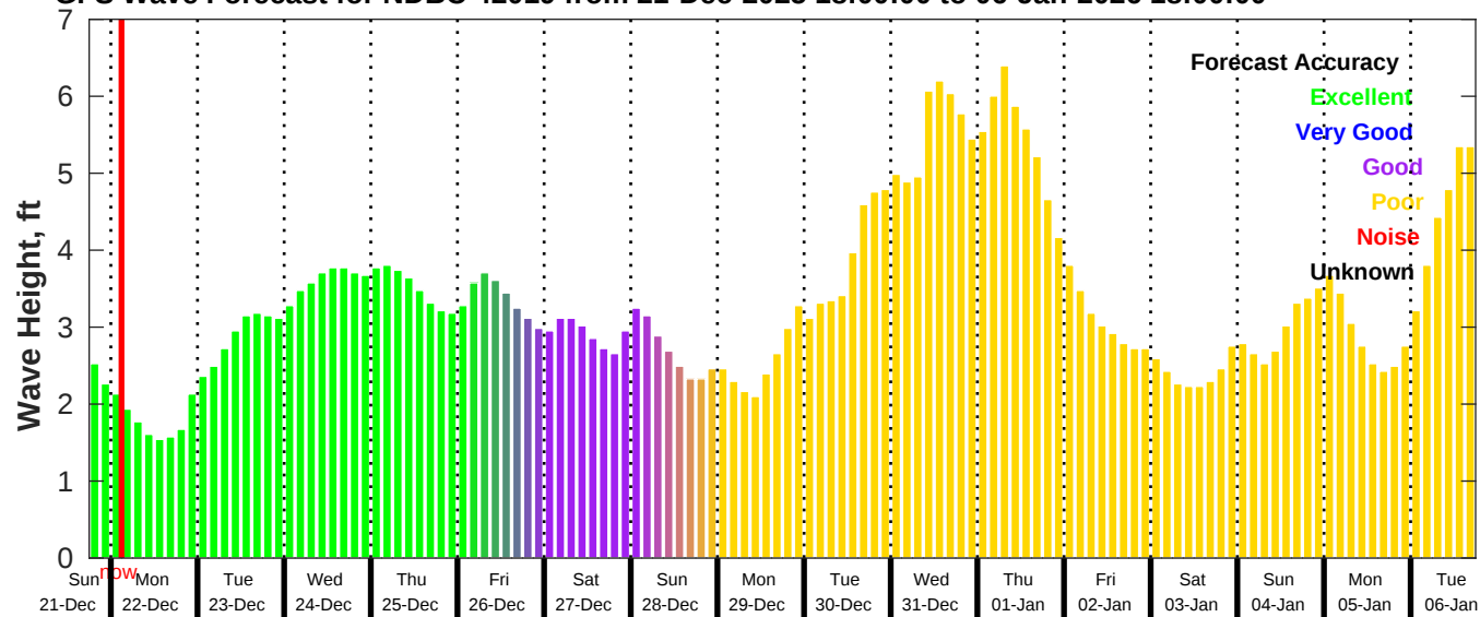
GFS Wave Forecast for NDBC 42019 from 21-Dec-2025 18:00:00 to 06-Jan-2026 18:00:00
