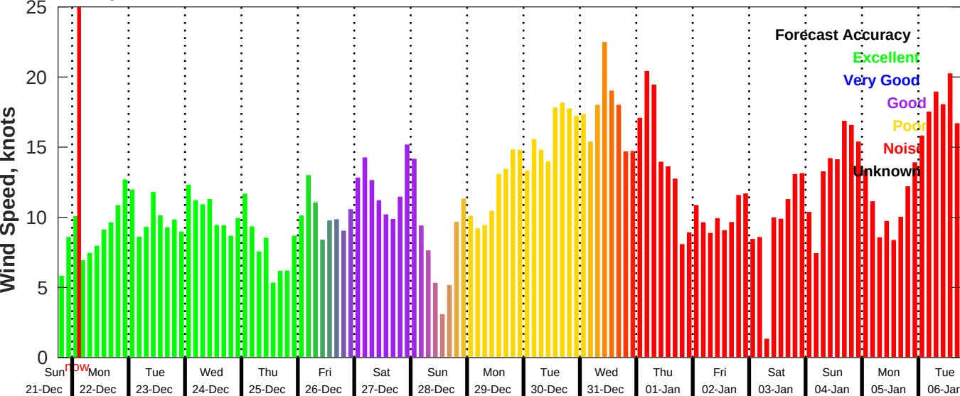
GFS Wind Speed Forecast for NDBC 42019 from 21-Dec-2025 18:00:00 to 06-Jan-2026 18:00:00
