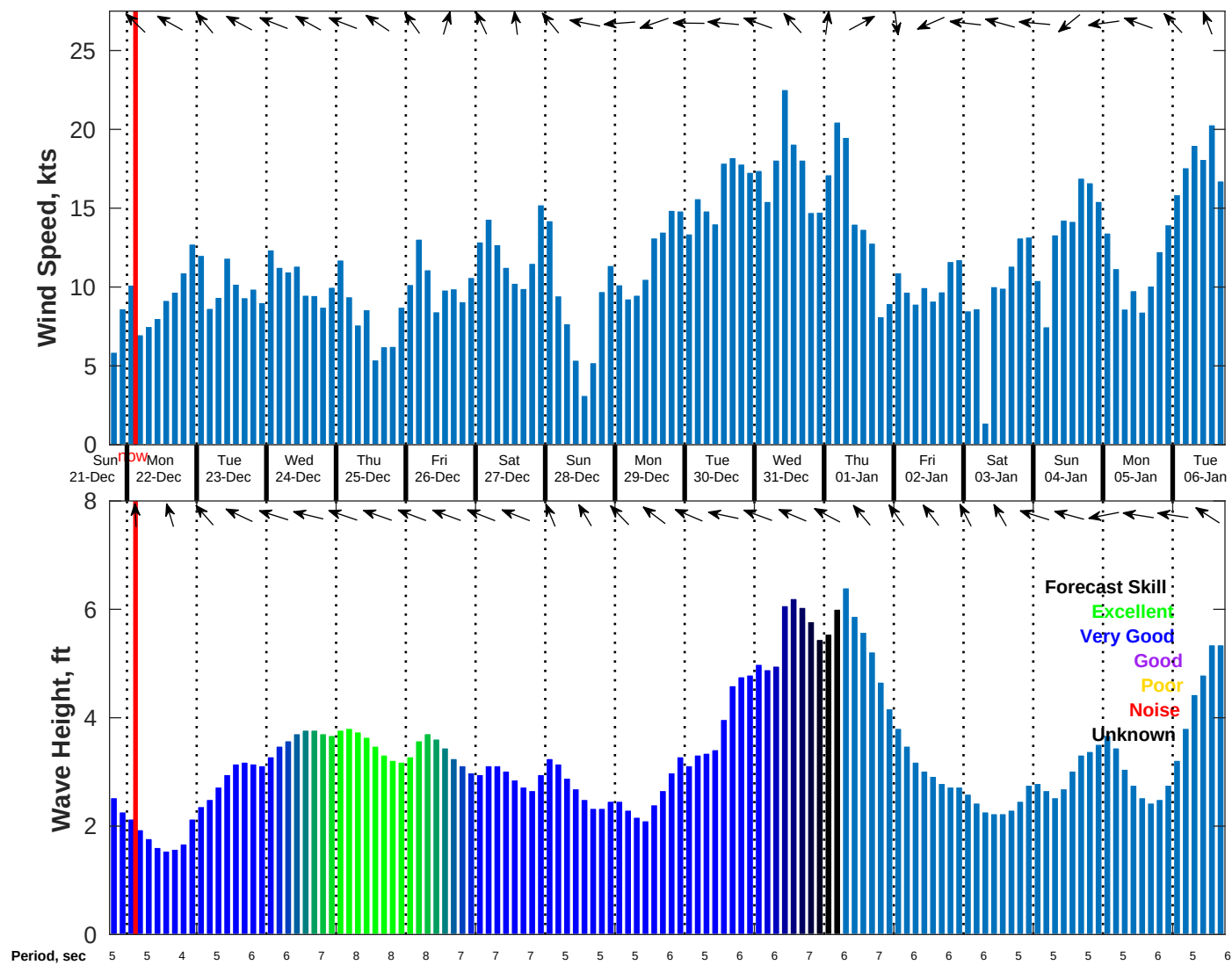
Wind & Wave Forecast for NDBC 42019 from 21-Dec-2025 18:00:00 to 06-Jan-2026 18:00:00
