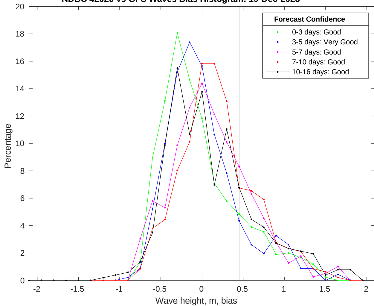
NDBC 42020 vs GFS Waves Bias Histogram: 19-Dec-2025
