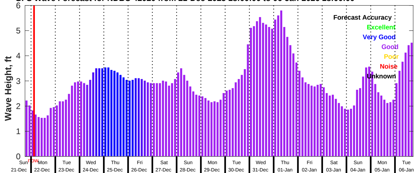
GFS Wave Forecast for NDBC 42020 from 21-Dec-2025 18:00:00 to 06-Jan-2026 18:00:00
