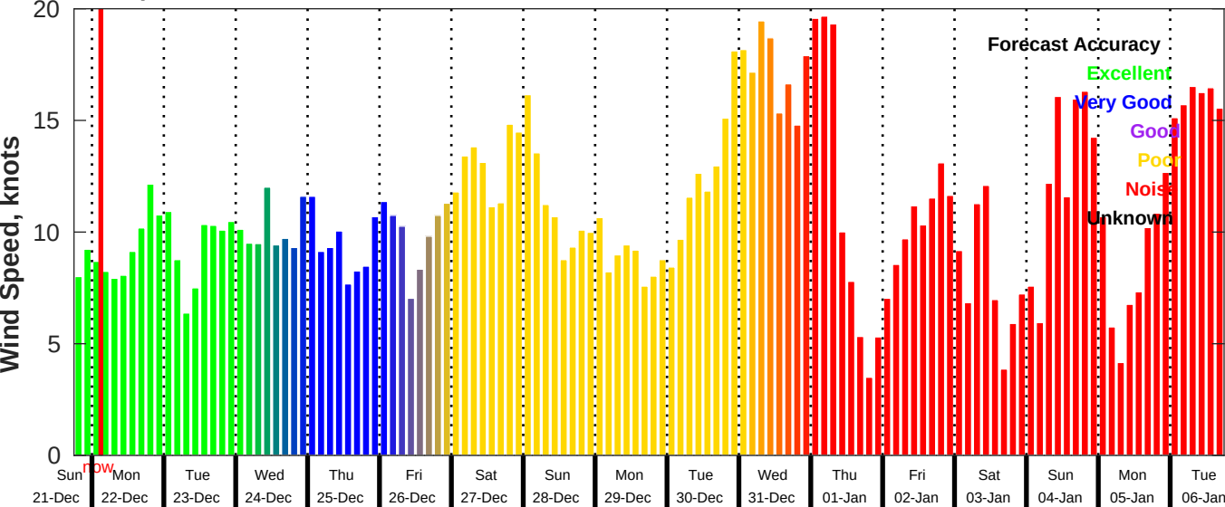
GFS Wind Speed Forecast for NDBC 42020 from 21-Dec-2025 18:00:00 to 06-Jan-2026 18:00:00
