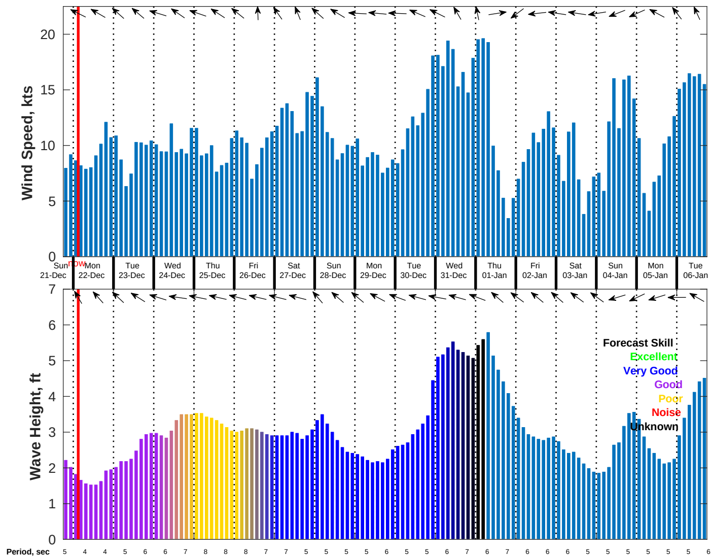
Wind & Wave Forecast for NDBC 42020 from 21-Dec-2025 18:00:00 to 06-Jan-2026 18:00:00
