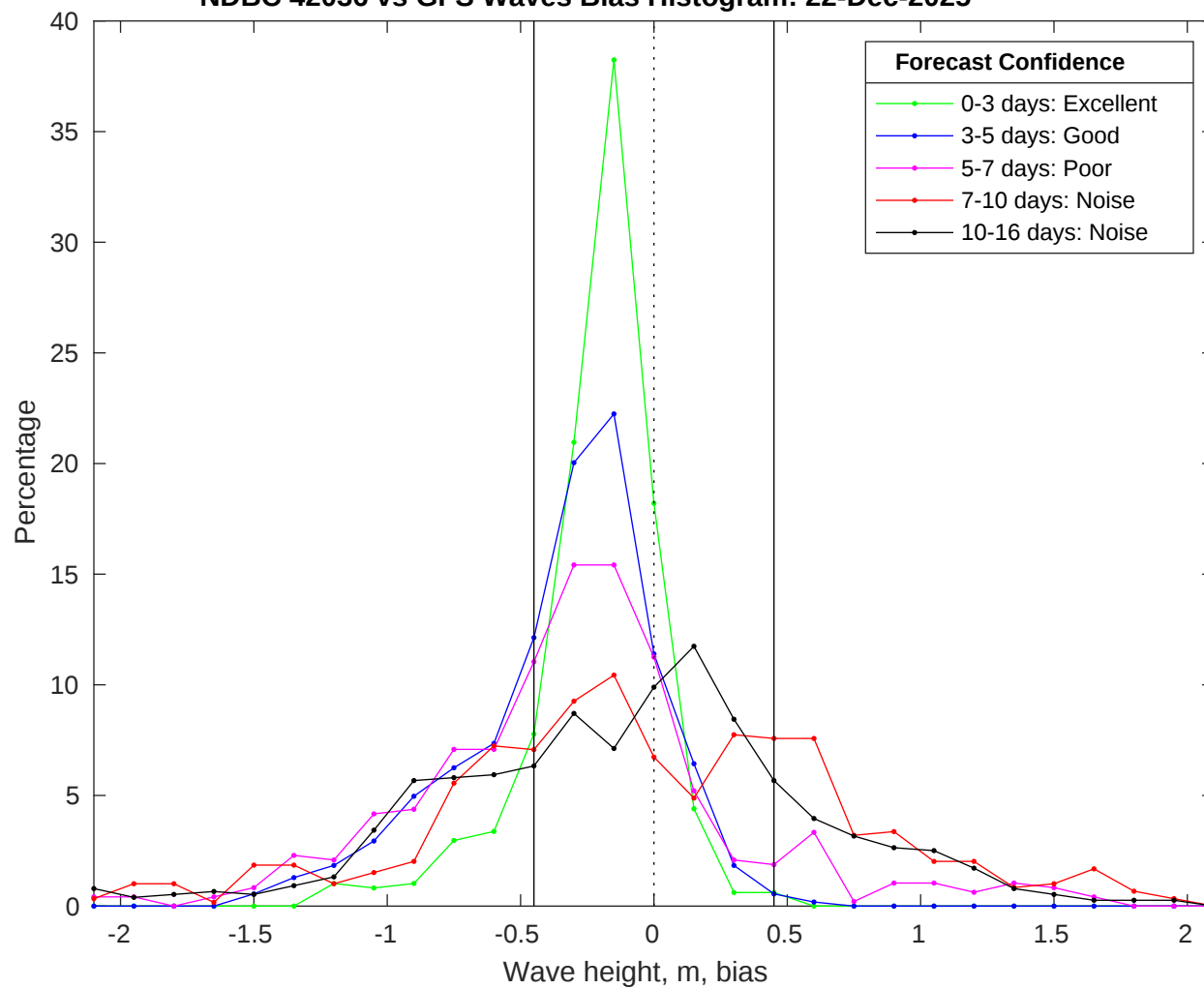
NDBC 42036 vs GFS Waves Bias Histogram: 22-Dec-2025
